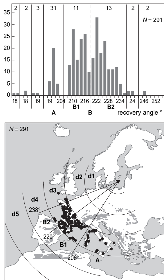
Fig. 3. Division of Robin recoveries from sector d3 of recovery distances 1201-1800 km. Top figure: frequency distribution for recovery angle – see text for how divisions were made; continuous line – first division, dashed line – secondary division, sample sizes at top of figure. Bottom figure – final division of recoveries from sector d3; continuous lines – divisions between groups verified by date criterion, groups B1 and B2 as on upper figure, group A enlarged to include adjacent low sample size groups. Marked in background are 600-km sectors (d1-d5) of recovery distances (dashed lines) and mean geographical location for the ringing stations (triangle). Other explanations as in Fig. 2.
