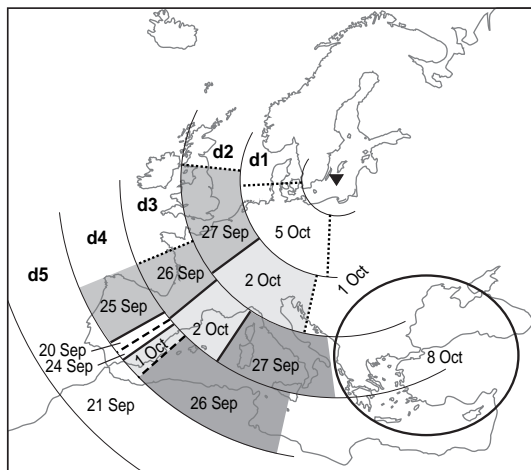
Fig. 4. Groups of recoveries distinguished in subsequent sectors and their mean dates (sample sizes in Table 3). Arches and symbols d1–d5 – sectors of recovery distance (see Fig. 2), thick line – divide between groups with mean migration date differing at P < 0.05 , dashed line – divide between groups with mean differing at 0.05 < P < 0.1 , dotted lines – borders of low-size groups not confirmed by statistical test, ellipse – delimitation of 'Balkan' group (see Fig. 2). Groups joined in series marked with the same fill pattern.
