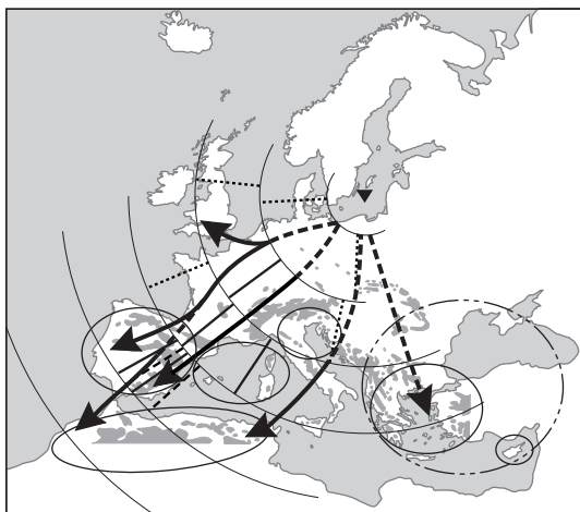
Fig. 6. Proposed course of migration routes against background of distinguished groups of recoveries (see Fig. 5) and glacial refugia. Thick continuous lines – course of migration routes documented by statistical tests (see text), thick dashed lines – hypothetical course, continuous line ellipses – ranges of glacial refugia (according to Harrison 1982, modified).
